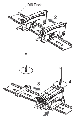
Tighten the screw while pressing the End Plate.
