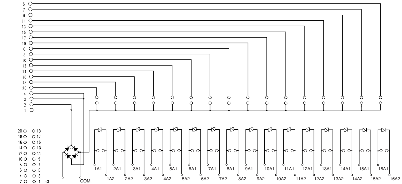
Connector Terminal Arrangement (Top View)
